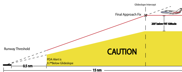
Figure 10-22 ILS Approach PDA Alert Threshold
