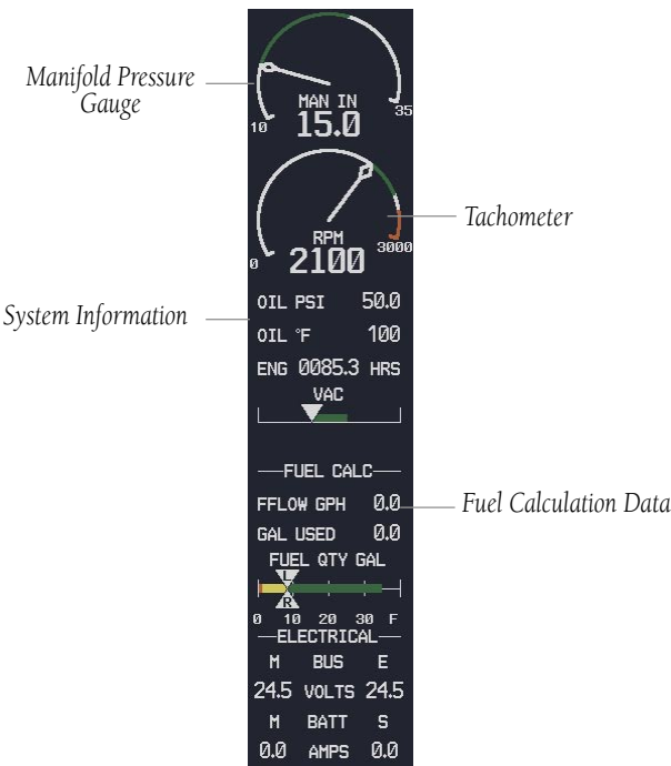
Figure 3-3 SYSTEM Engine Page (206H Shown)
