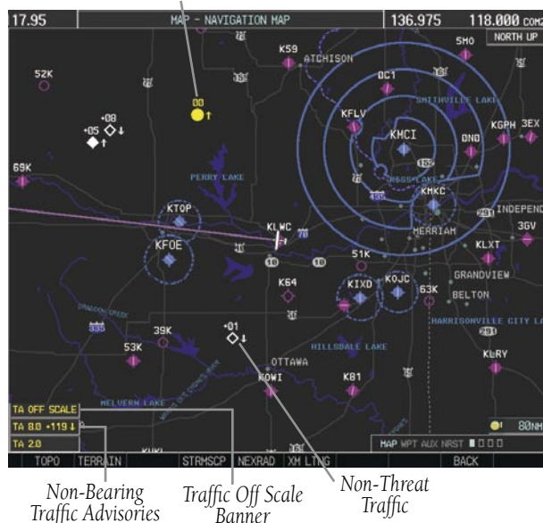
Figure 10-14 TAS Traffic on Navigation Map
