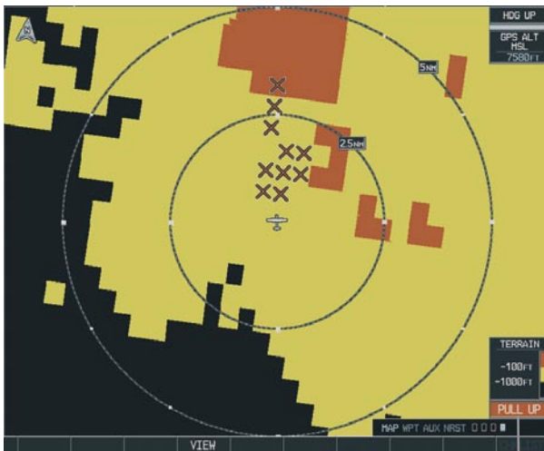
Figure 10-27 Alert Annunciation on the TAWS Page
