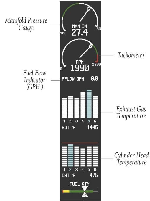
Figure 3-2 LEAN Engine Page (182T Shown)
