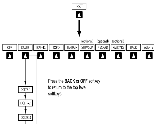
Figure 1-3 PFD Softkey Flow Chart – 1
