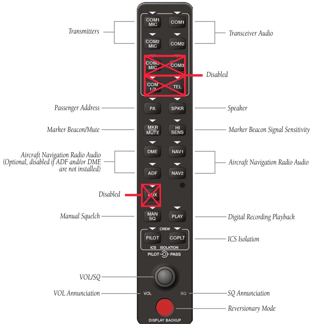
Figure 5-1 Front Panel Controls
