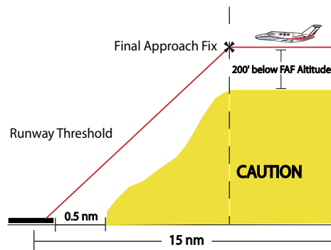
Figure 10-21 Non-Precision Approach PDA Alert Threshold
