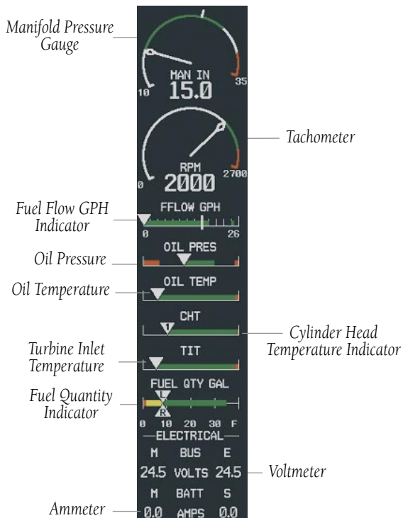
Figure 3-1 Default Engine Page (T182T Shown)
