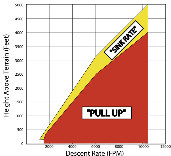
Figure 10-23 Excessive Descent Rate
